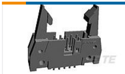
TE Part #1-102321-2 064 UNIV HDR SP 4S 30DP STD L1
