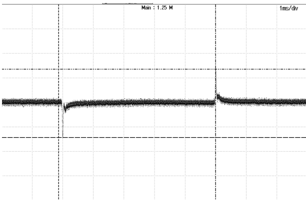
Figure 7: Output voltage response to step-change in load current (50%-75%-50% of full load; di/dt = 0.1A/\mu s ). Bottom Trace: V_{out} ; 100mV/div; Time: 1ms/div
