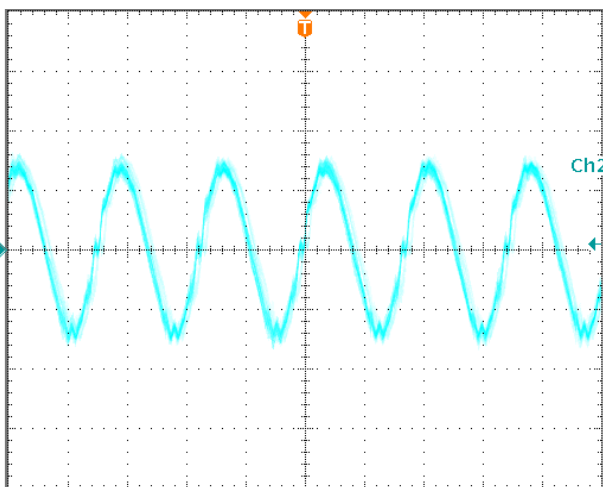
Figure 10: Output voltage ripple at nominal input voltage and max load current (10 mV/div, 2μs/div) Bandwidth: 20 MHz.
