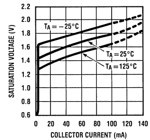
Saturation Voltage
