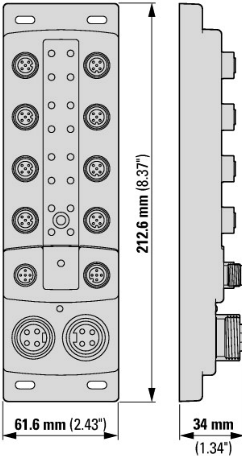
SmartWire-DT I/O modules, EU8E-SWD-... block module with external supply
