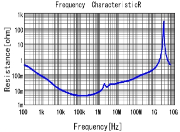
■ KCM55WR72A156MH01 R DCOV, 25degC
