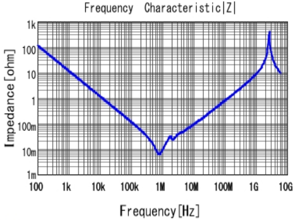
■ KCM55WR72A156MH01 |Z| DCOV, 25degC
