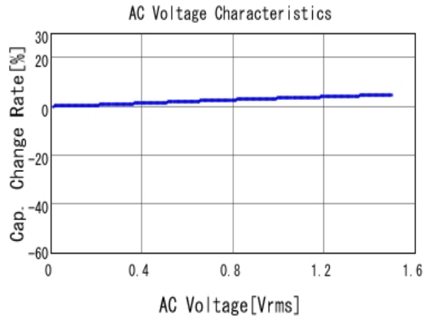
■ KCM55WR72A156MH01 C-AC Voltage capchange, DCOV, 25.0d
