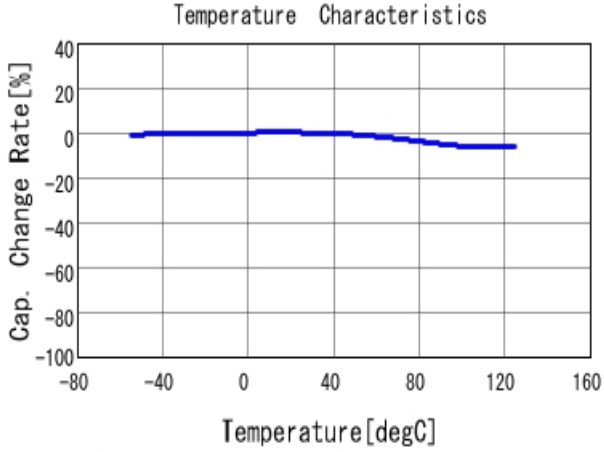
■ KCM55WR72A156MH01 C-Temp. capchange, DCOV, ACO, 5Vrms
