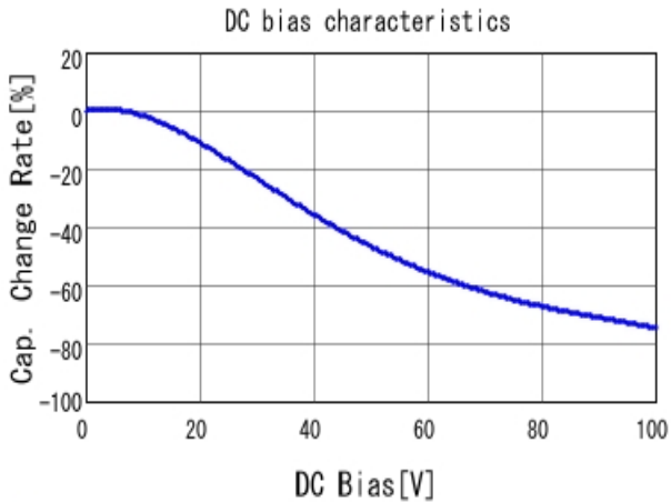
■ KCM55WR72A156MH01 C-DC bias capchange, 25.0degC, AC0.
