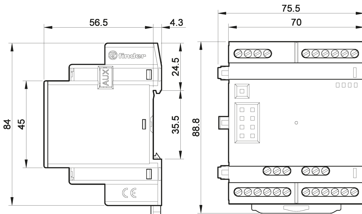
Arduino Opta® Analog Expansion Outline. Dimensions are in mm
