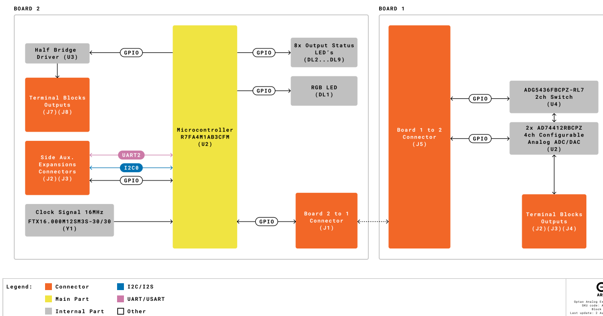
Block diagram
