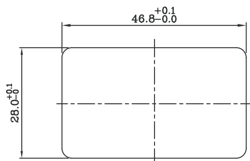
PANEL CUT-OUT
