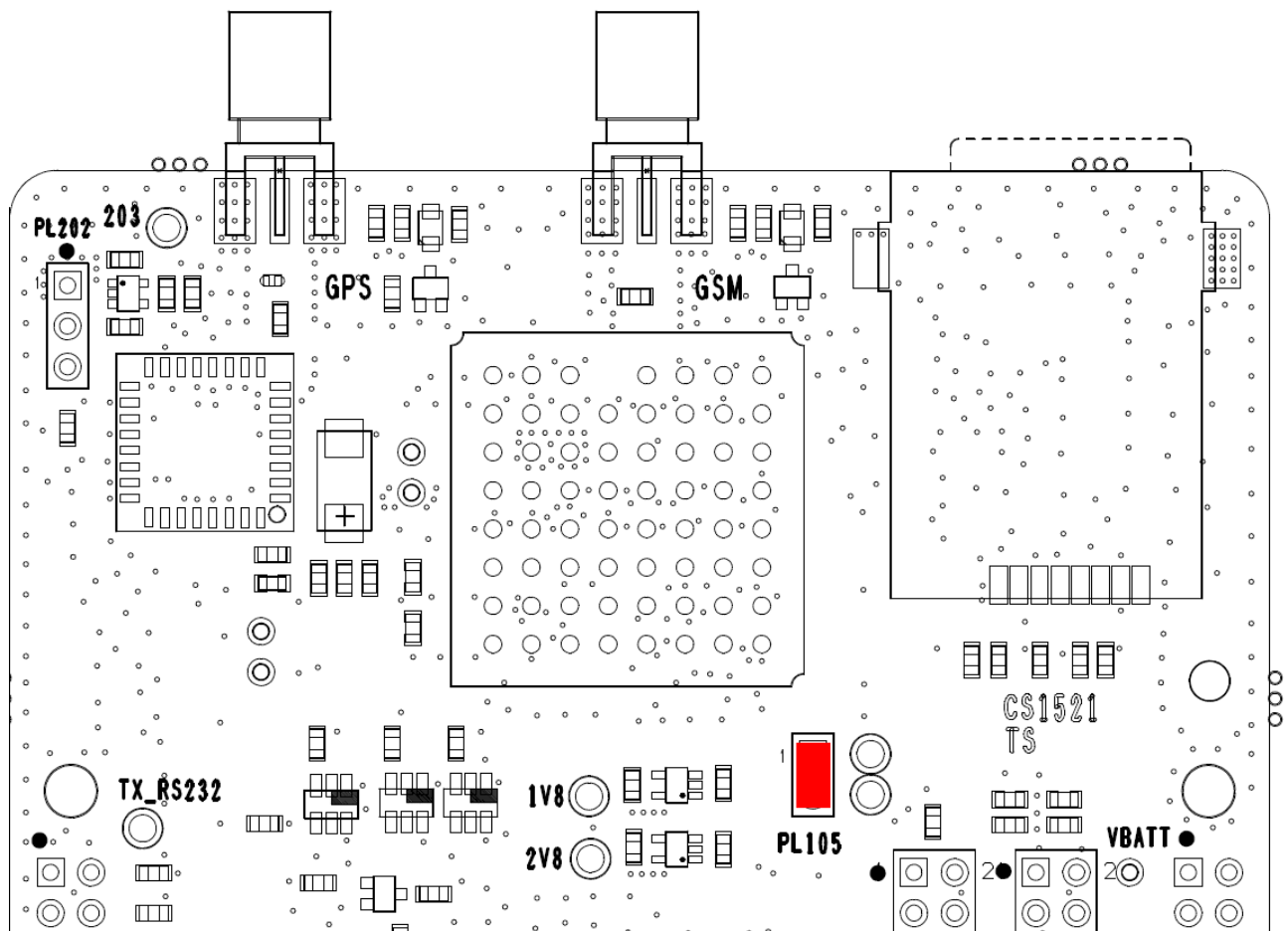
Figure 47. Jumper for VBATT.
