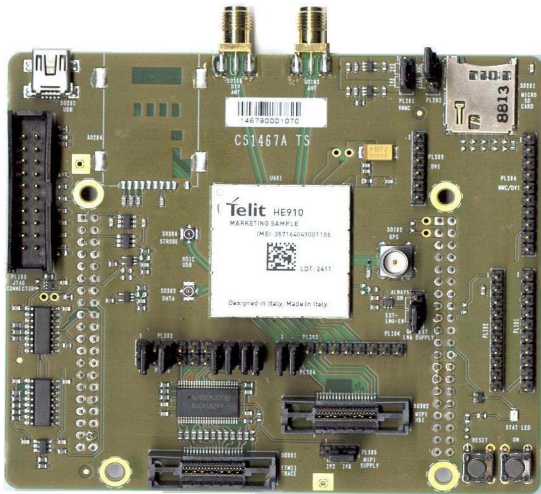
Interface Board
