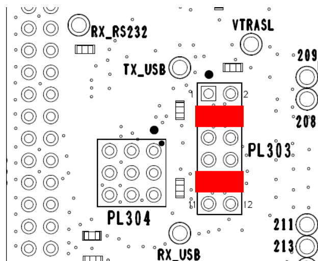
Figure 53.GPS to USB
