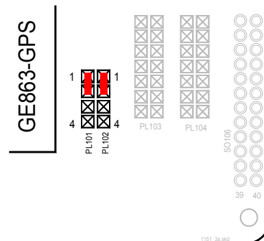
Figure 27: Jumpers setting for GE863-PY/QUAD
