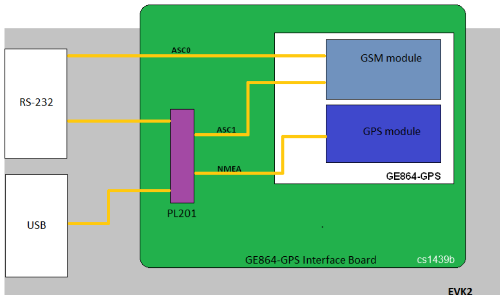
Figure 34. GE864-GPS Interface Board serial connections
