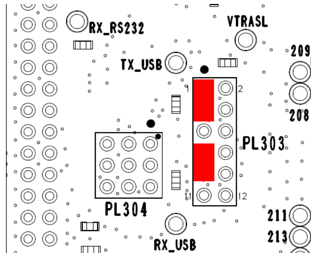
Figure 52.GSM to USB
