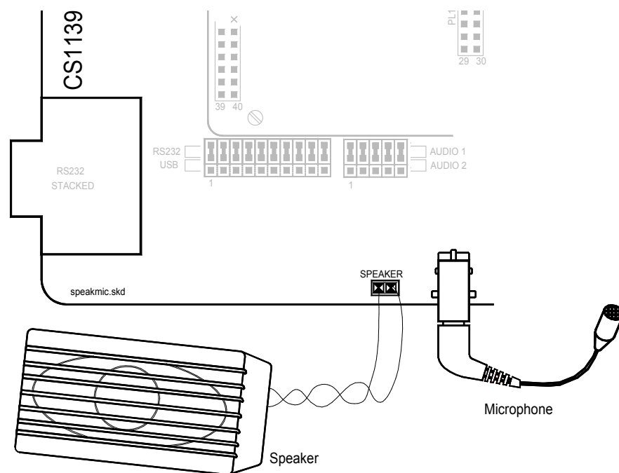
Figure 18: Speaker &amp; Microphone case insertion
