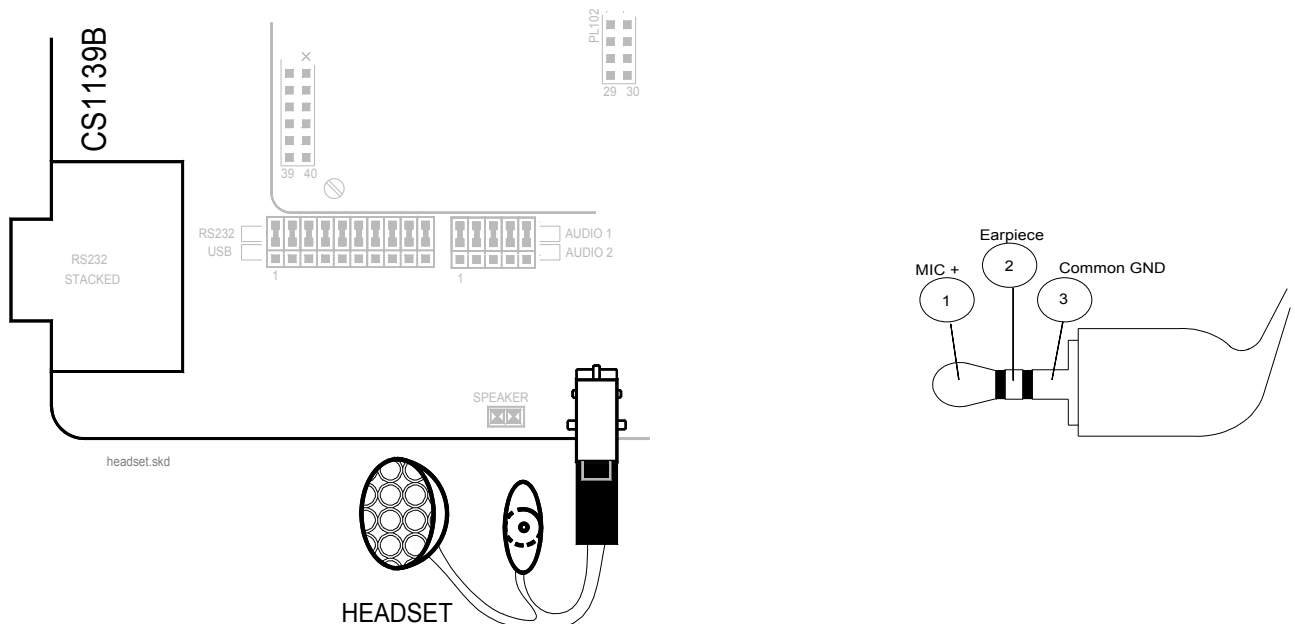
Figure 14: Headset insertion
