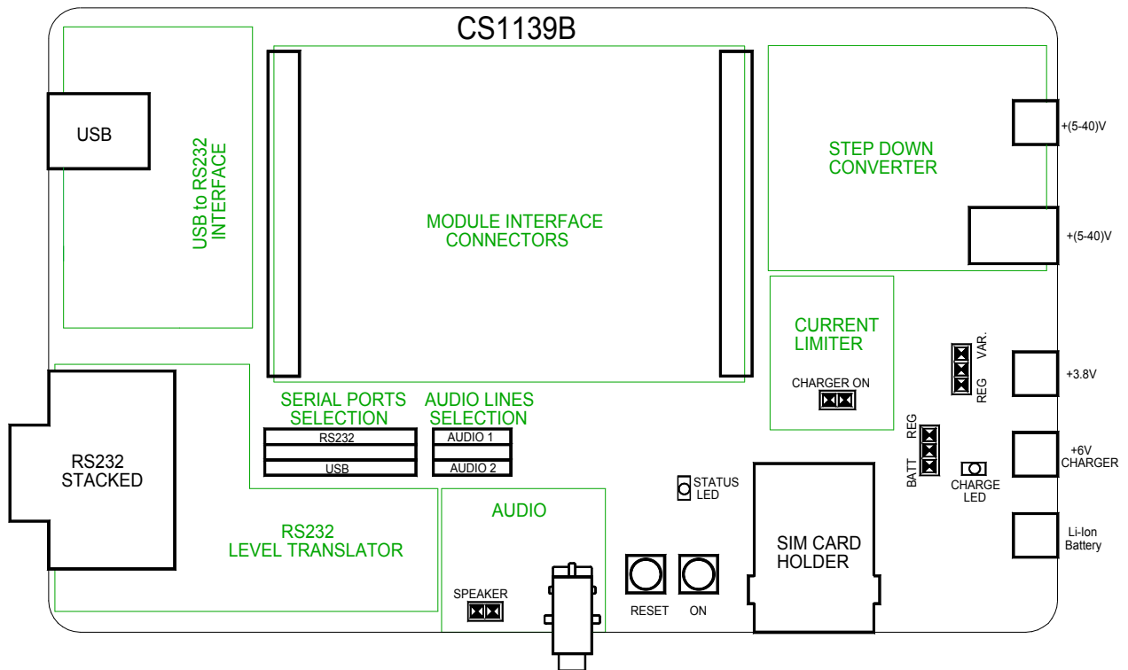
Figure 3: CS1139B circuital displacement
