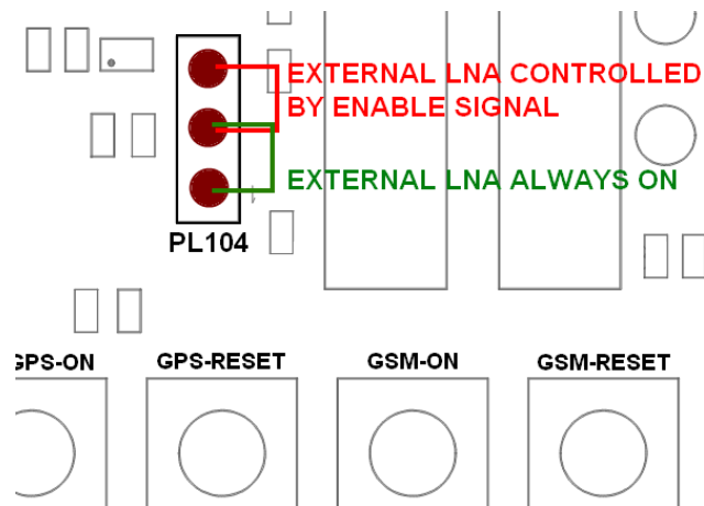
Figure 33. Jumper on PL104.
