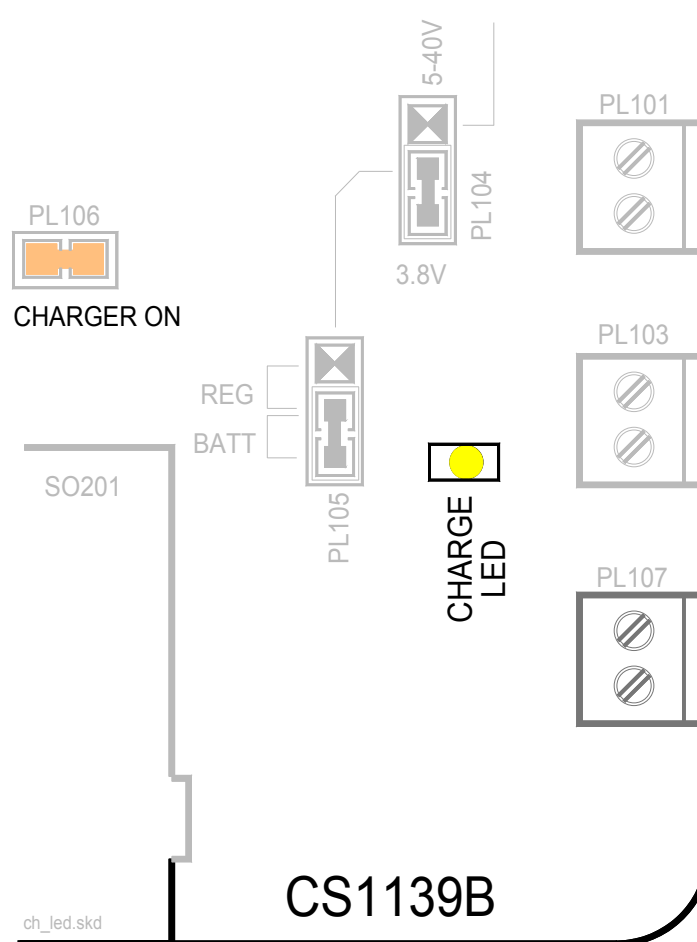
Figure 21: CHARGE LED position
