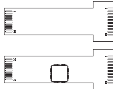
PCB Pin Assignment
