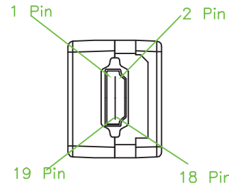
HDMI Female (Out Put)
