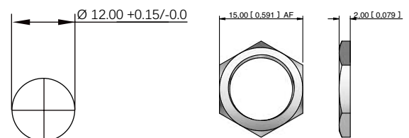
PANEL CUTOUT
