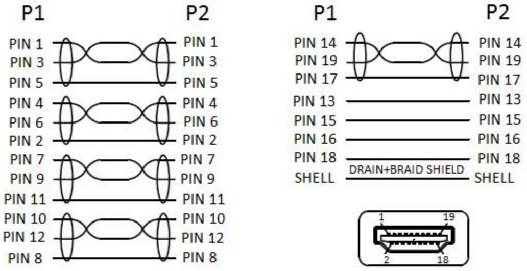
Pin Assignment
