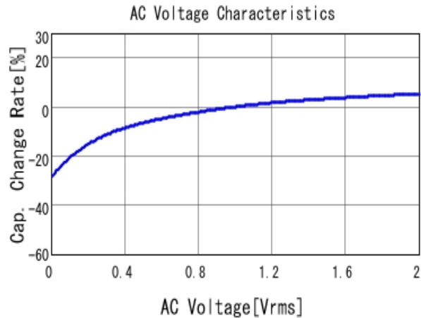
■ GRM033C81E104ME14 C-AC Voltage capchange, DCOV, 25.0d
