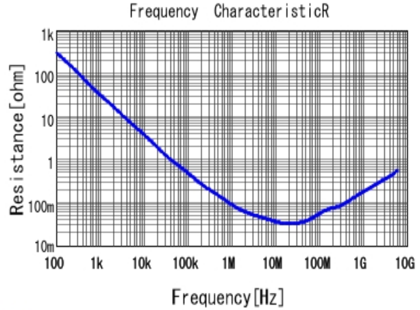
■ GRM033C81E104ME14 R DCOV, 25degC
