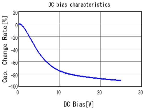
■ GRM033C81E104ME14 C-DC bias capchange, 25.0degC, AC1V
