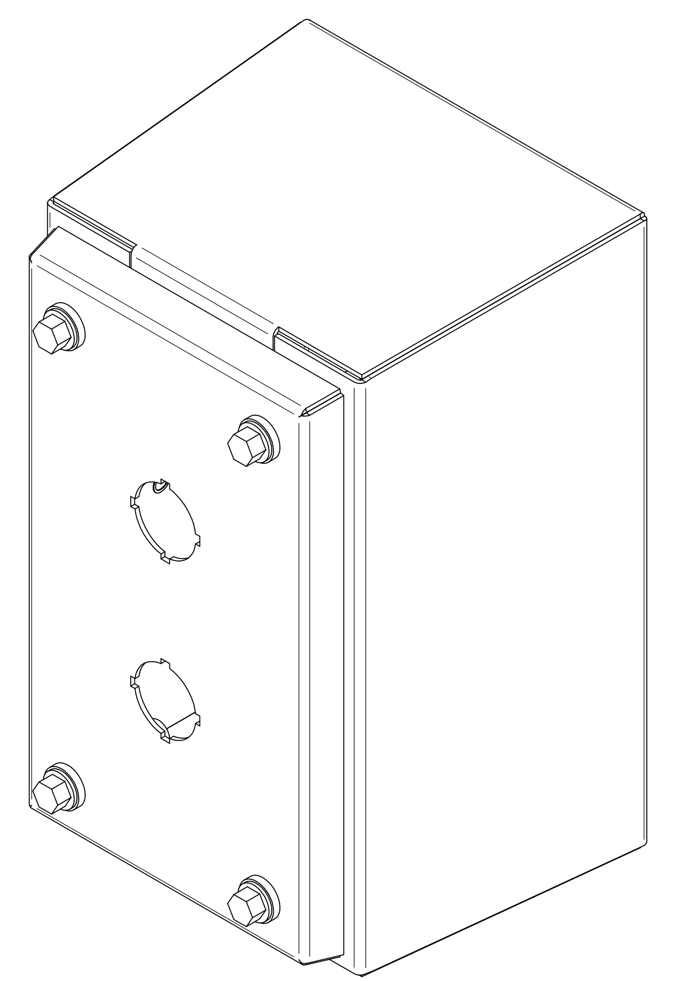
ISOMETRIC VIEWS
