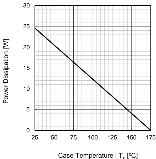
Fig.6 Power Dissipation
