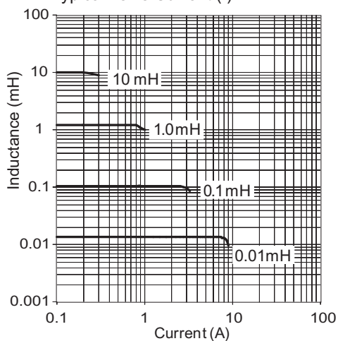
Typical Ls vs Current (I)
