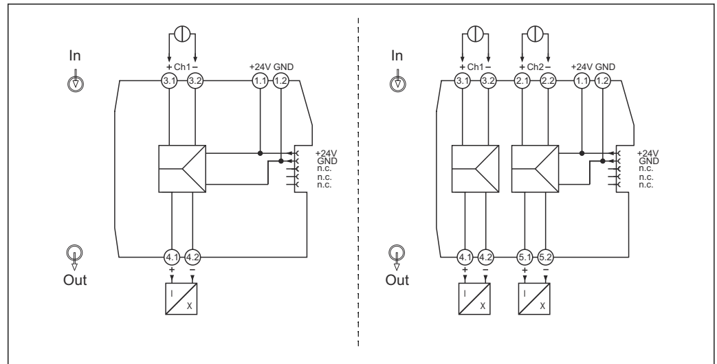
8 Terminal assignment of RNO22: 1-channel version (left), 2-channel version (right)
