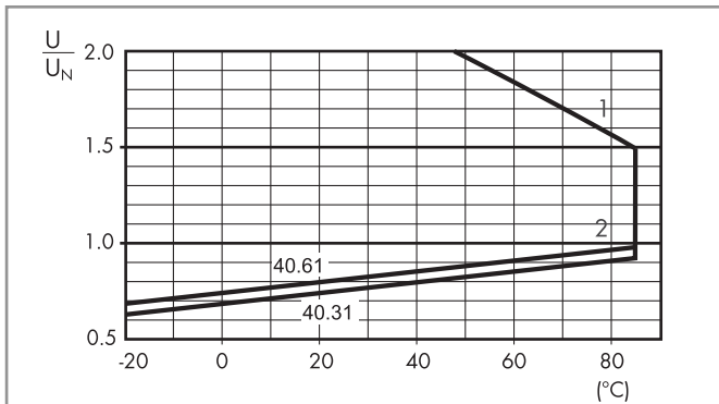
R 40 - DC coil operating range v ambient temperature
