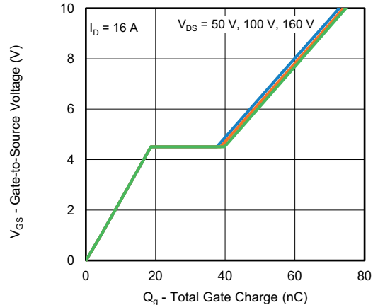
Gate Charge
