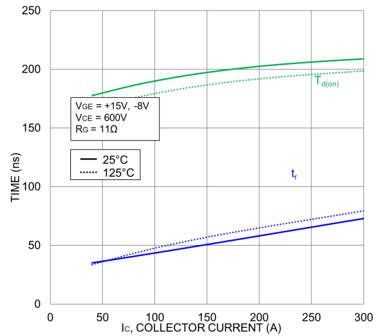
Figure 14. Typical Turn-On Switching Time vs. IC
