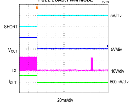
MAXM17905 OUTPUT SHORT IN STEADY STATE V_{IN} = 12V , FIXED V_{OUT} = 5V , FULL LOAD, PWM MODE
