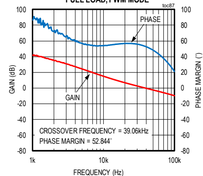
MAXM17906 BODE PLOT V_{IN} = 12V , ADJUSTABLE V_{OUT} = 5V , FULL LOAD, PWM MODE
