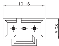
(3 Pin)
