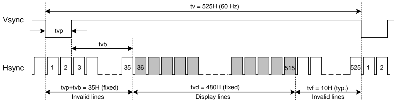
Fig. 9.2 Vertical Timing
