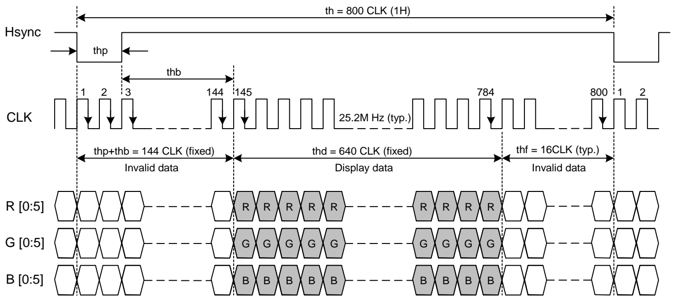
Fig. 9.1 Horizontal Timing
