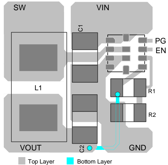
Figure 3: Recommended PCB Layout
