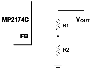
Figure 2: Feedback Network
