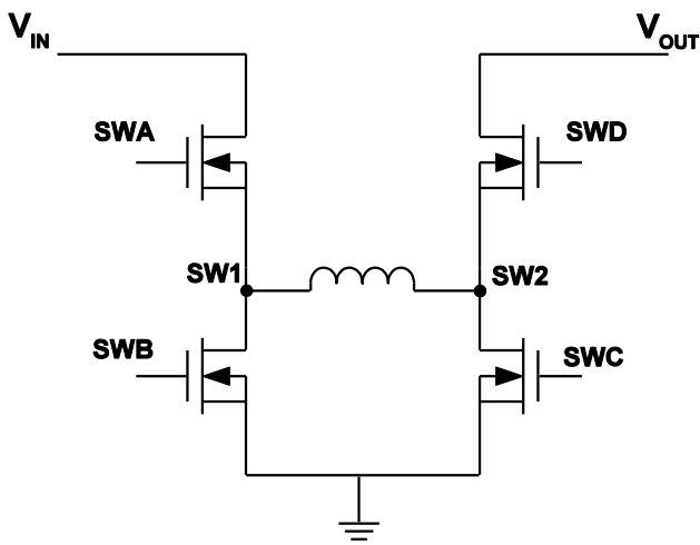
Figure 2: Buck-Boost Topology
