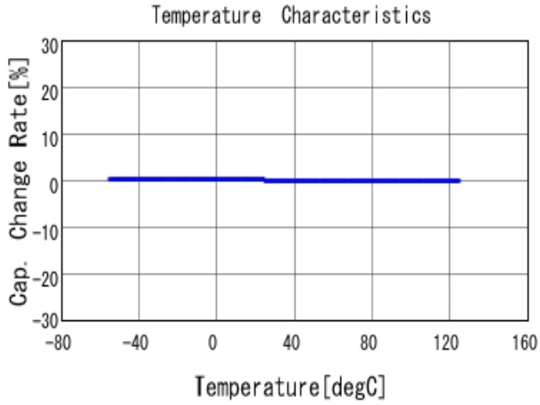
■ GCM0335C1H820FA16 C-Temp. capchange, DCOV, AC1Vrms
