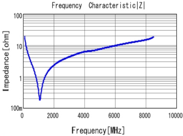
GCM0335C1H820FA16 |Z| DC0V, 25degC
