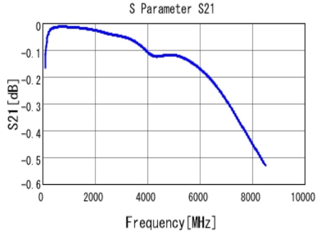
■ GCM0335C1H820FA16 S21 DCOV, 25degC
