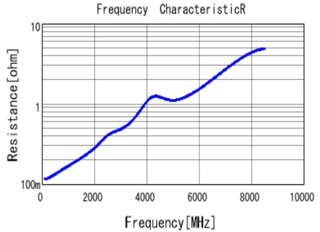
GCM0335C1H820FA16 R DC0V, 25degC
