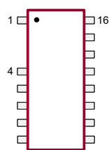
16-Lead SOIC
