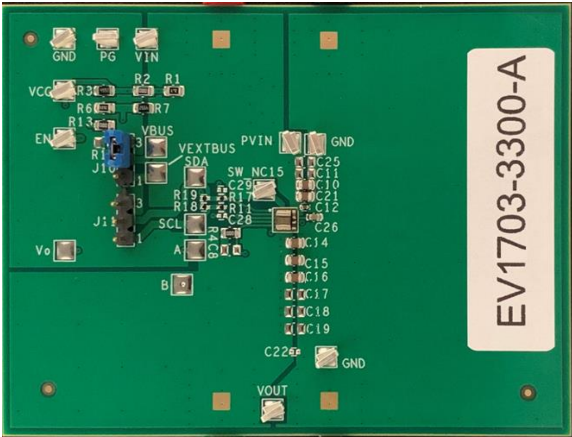
Figure 1 Board layout
