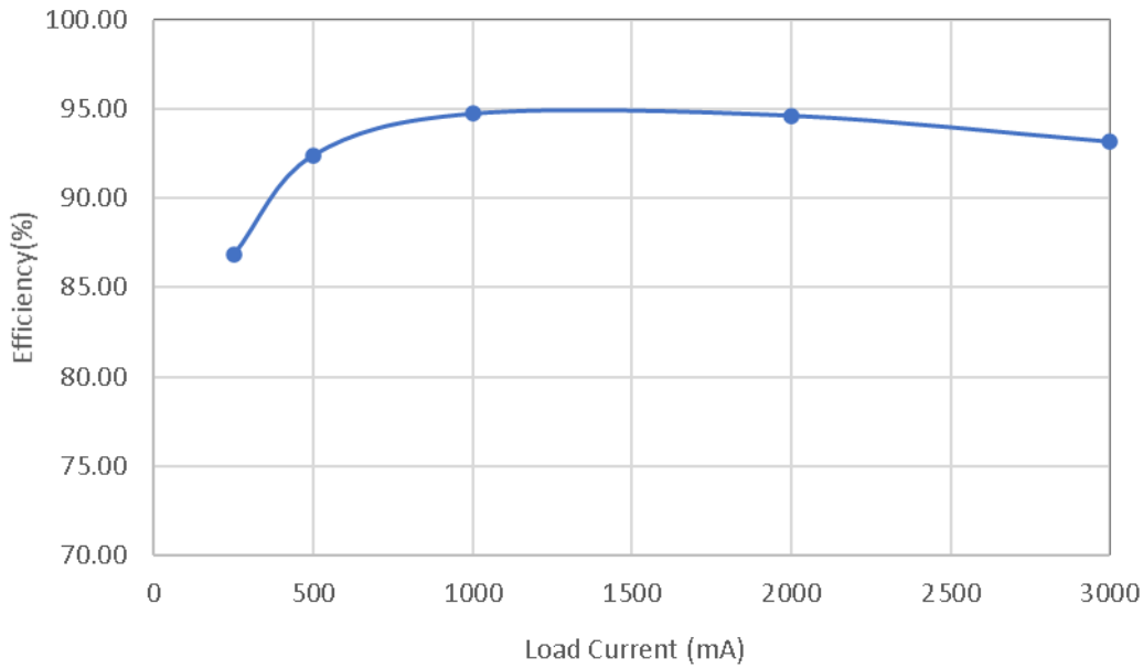
Figure 12 Efficiency
