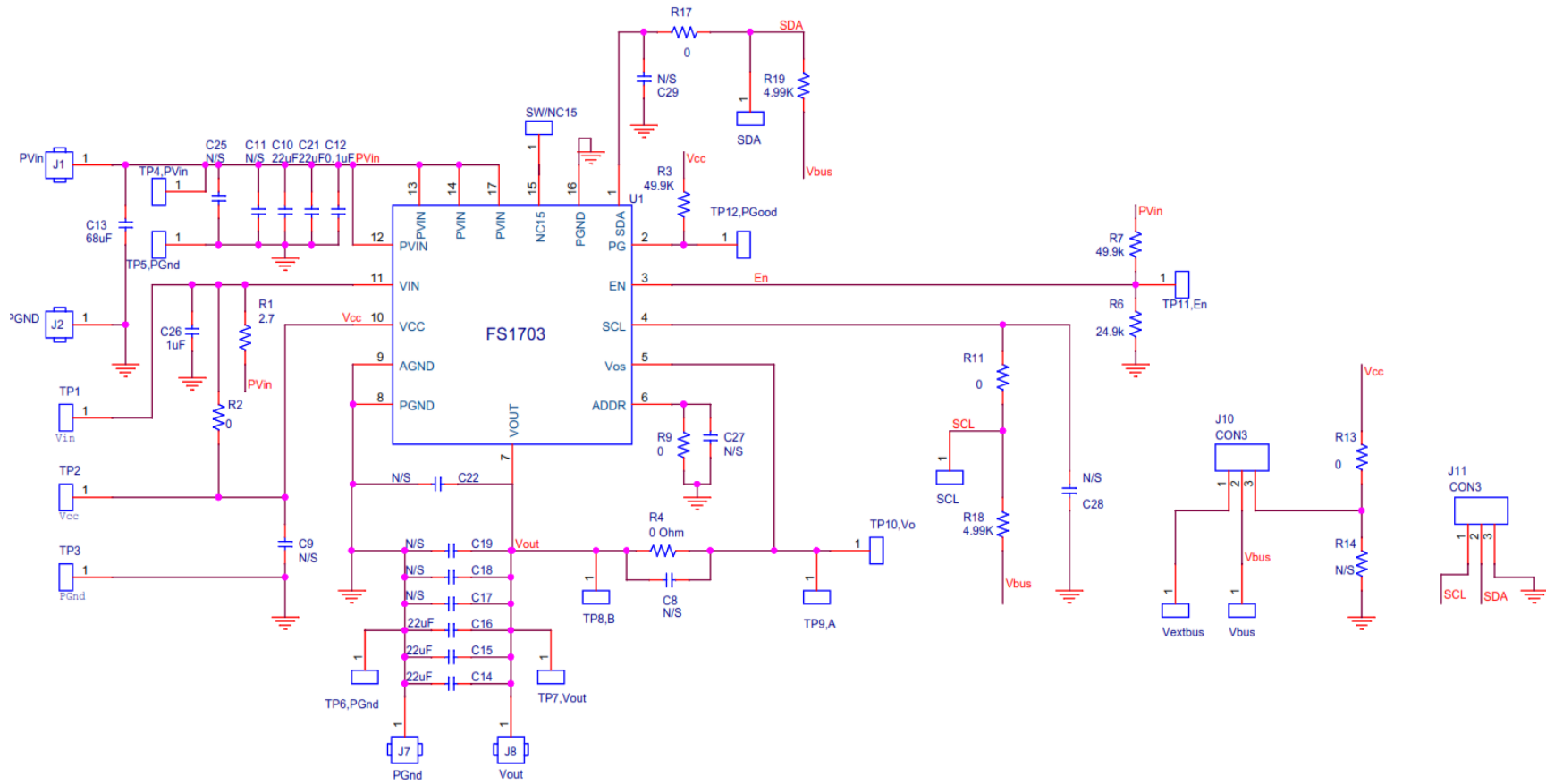
Figure 2 Schematic
