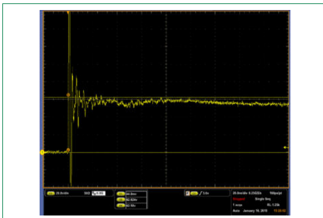
ISO10605 (C:330pF, R:330 \Omega ) contact discharge plot at +8KV
