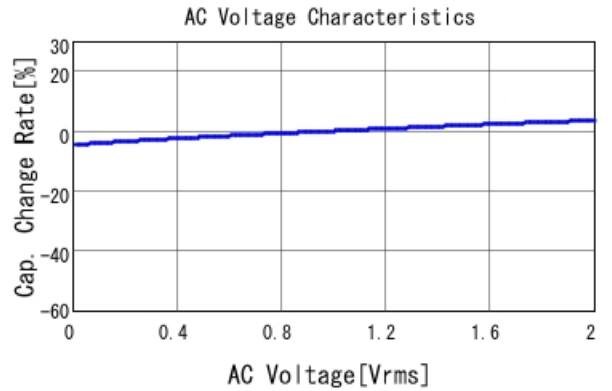
■ GCJ31CC72A225KE01 C-AC Voltage capchange, DC0V, 25.0d
