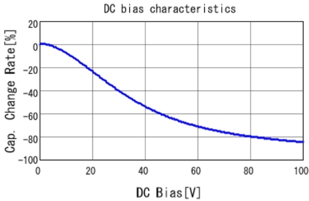
■ GCJ31CC72A225KE01 C-DC bias capchange, 25.0degC, AC1.
