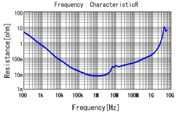
■ GCJ31CC72A225KE01 R DC0V, 25degC
