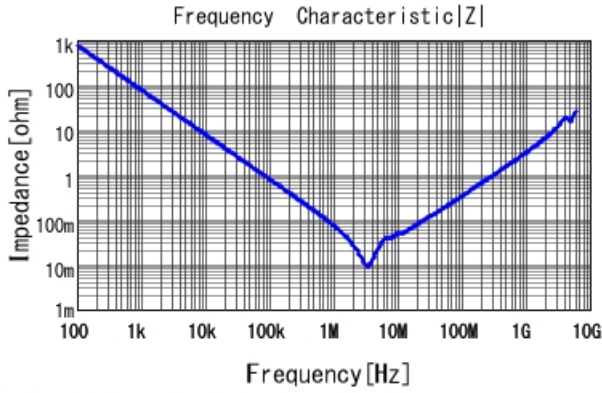
■ GCJ31CC72A225KE01 |Z| DC0V, 25degC
