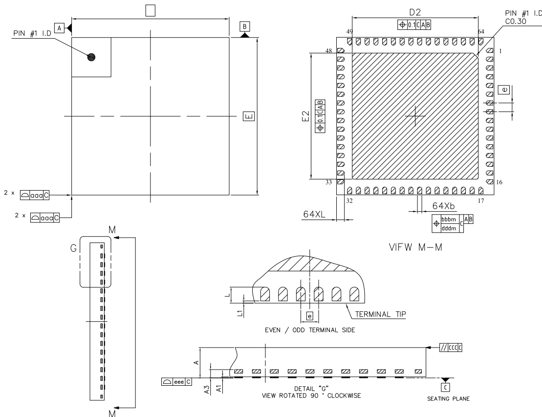
Figure 4.2. QFN64
