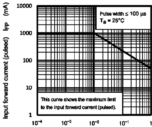
Duty cycle ratio D_R Fig. 11.3 I_{FP} - D_R
