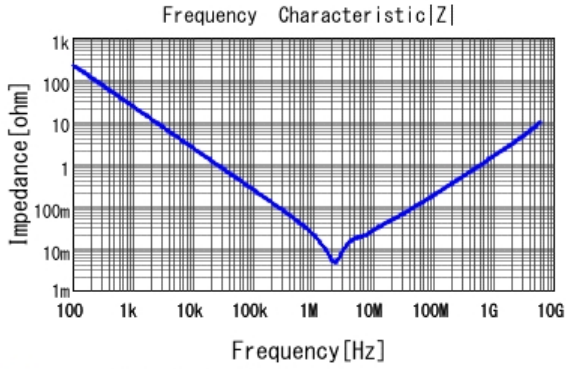
■ GRM188R61E106MA73 |Z| DCOV, 25degC
