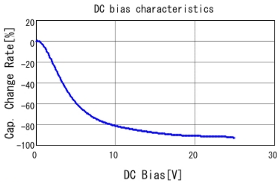
■ GRM188R61E106MA73 C-DC bias capchange, 25.0degC, AC1V
