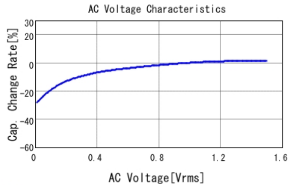
■ GRM188R61E106MA73 C-AC Voltage capchange, DCOV, 25.0d
