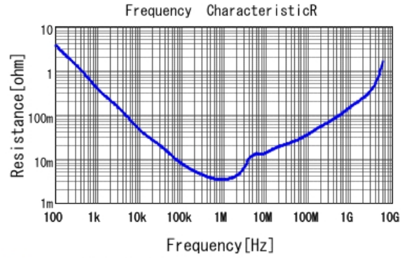
■ GRM188R61E106MA73 R DCOV, 25degC
