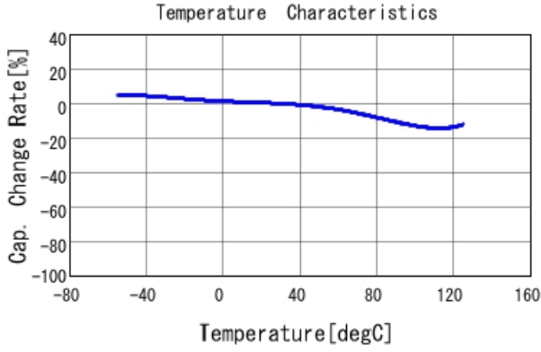
■ GRM43DR72E334KW01 C-Temp. capchange, DCOV, AC1Vrms
