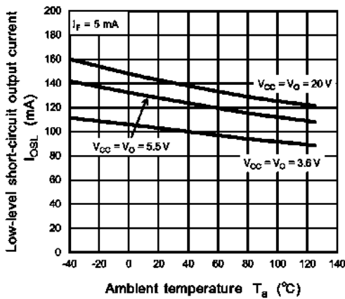
Fig. 12.2.9 I_{OSL} - T_a
