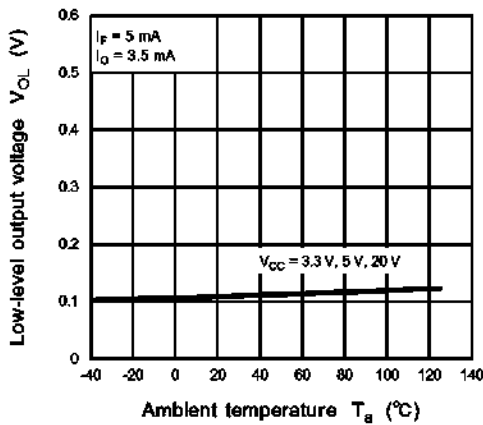
Fig. 12.2.3 V_{OL} - T_a
