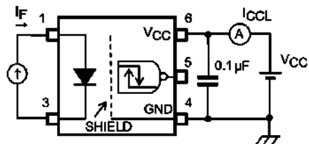
Fig. 12.1.3 I_{CCL} Test Circuit
