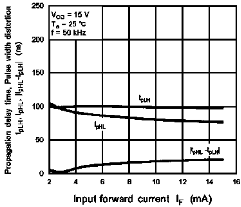
Fig. 12.2.19 t_{pHL}, t_{pLH}, |t_{pHL} - t_{pLH}| - I_F
