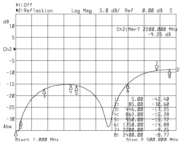
Top: Return loss
