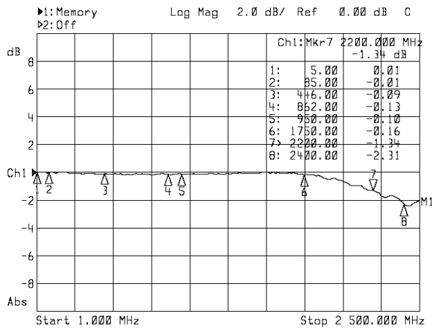
Top: Insertion loss
