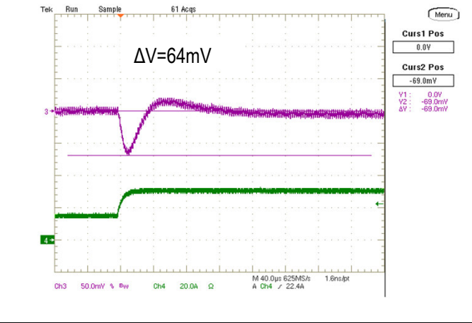
Step Load Transient Response (Vin=5.0V, Vout=1.8V, Cloud=760uF, Iout=15 to 30A, 1.0A/us) Trace 3=Vout, 50mV/div, Trace 4=Iout, 20A/div.
