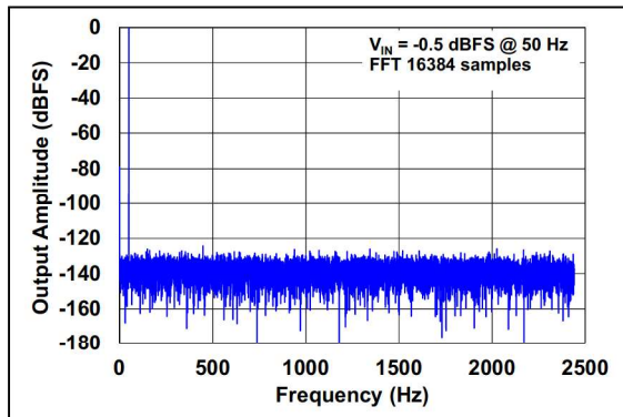
FIGURE 2-1: FFT Output Spectrum, f_{in} = 50 Hz Input.
