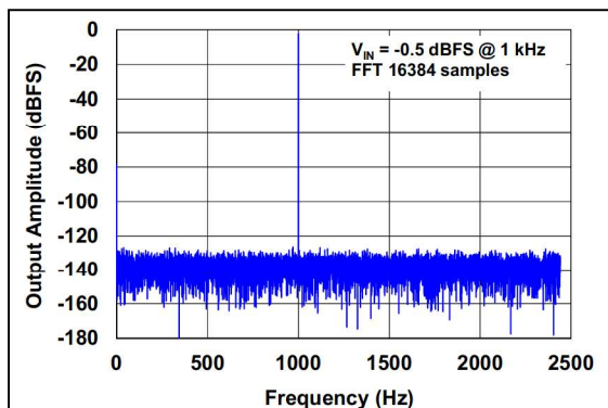
FIGURE 2-2: FFT Output Spectrum, f_{in} = 1 kHz Input.
