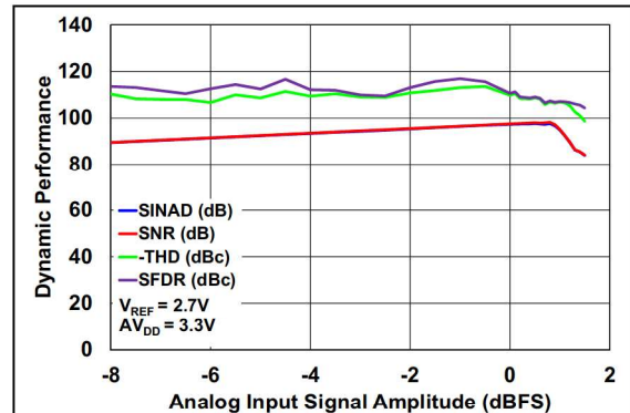
FIGURE 2-34: Dynamic Performance vs. Input Signal Amplitude.
