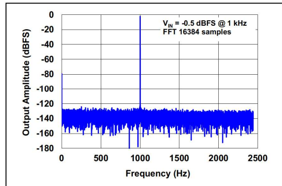
FIGURE 2-4: FFT Output Spectrum, f_{in} = 1 kHz (Internal V_{REF} ).
