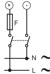
Fig. 17 Auxiliary power supply (H). 250 V [T] 630 mA fuse (F).
