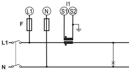
Fig. 15 Single-phase system (2-wire), 1 CT. 315 mA fuse (F).
