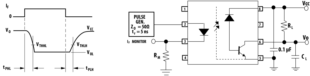
Figure 12: Switching Test Circuits
