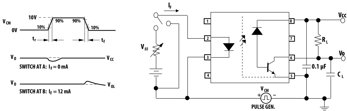
Figure 13: Test Circuit for Transient Immunity and Typical Waveforms
