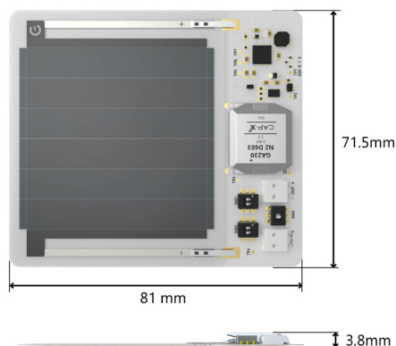
Mechanical Dimensions
