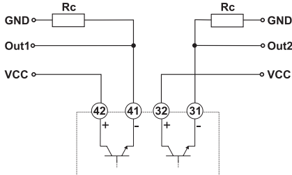
Fig. 26 Static outputs, VCC reference
