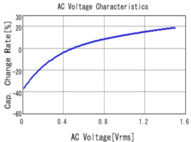
■ GCJ31CR71A226KE01 C-AC Voltage capchange, DCOV, 25.0d
