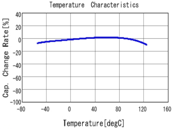
■ GCJ31CR71A226KE01 C-Temp. capchange, DC0.0V, AC0.5V rm
