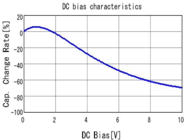
■ GCJ31CR71A226KE01 C-DC bias capchange, 25.0degC, AC0.
