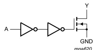
Fig 3. Logic diagram
