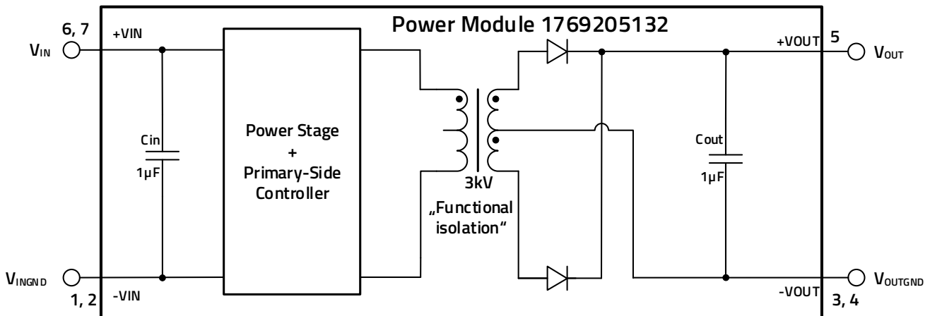
Figure 10: 1769205132 block diagram.
