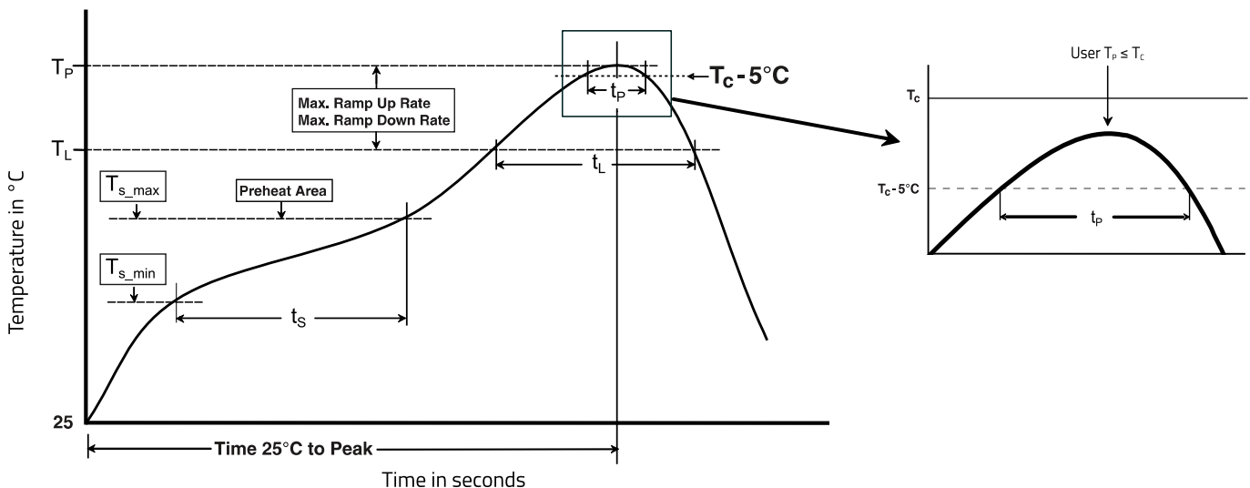
Figure 18: Soldering profile.
