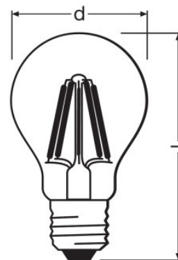
PARATHOM Retrofit CLASSIC A 60 6 W/827 E27, P RF CLAS A 60 6 W/827 E27, P RF CLAS A 75 8 W/827 E27
