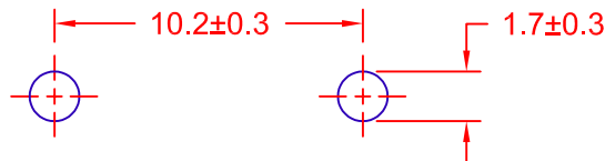
PC-BOARD PATTERN
