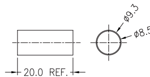
INSULATION TUBE
