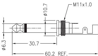
BODY
