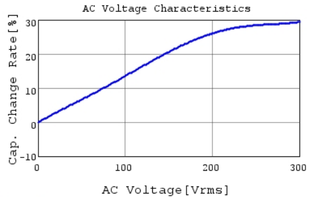
DE1E3RA472MN4AP01F C-AC Voltage capchange, I
