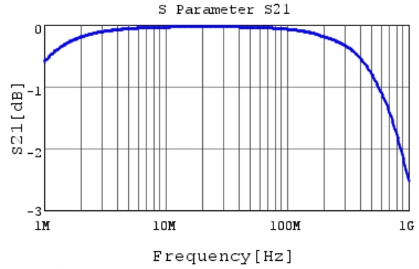
DE1E3RA472MN4AP01F S21 DCOV, 20degC
