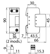
Dimension drawing DGP M 255 FM
