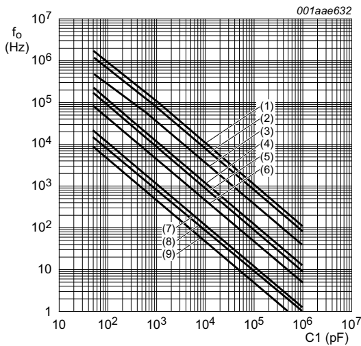
T amb = 25 °C; VCO_IN at 0.5V DD ; INH_IN at V SS ; R2 = ∞. Lines (1), (4), and (7): V DD = 15 V; Lines (2), (5), and (8): V DD = 10 V; Lines (3), (6), and (9): V DD = 5 V; Lines (1), (2), and (3): R1 = 10 kΩ; Lines (4), (5), and (6): R1 = 100 kΩ; Lines (7), (8), and (9): R1 = 1 MΩ.
